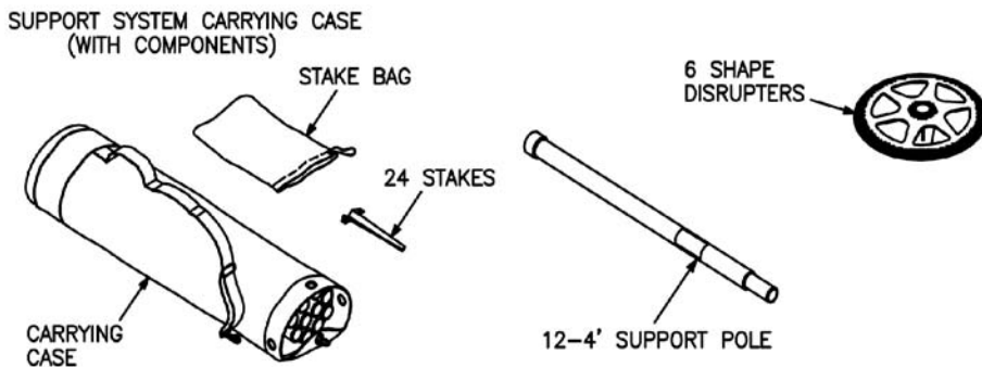
Figure 1-2. ULCANS Components
